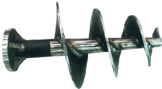
大小頭擠壓螺旋桿 Big head and small head extruding screw
