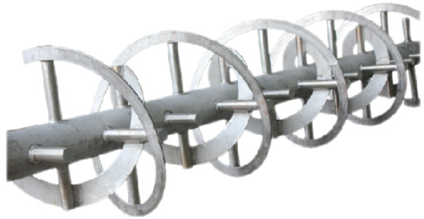
攪拌式螺旋桿 Mix-type screw
