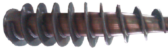
大小頭擠壓螺旋桿 Big head and small head extruding screw
